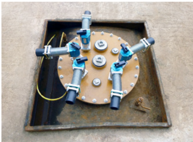
Tank surface being prepared for bonding
