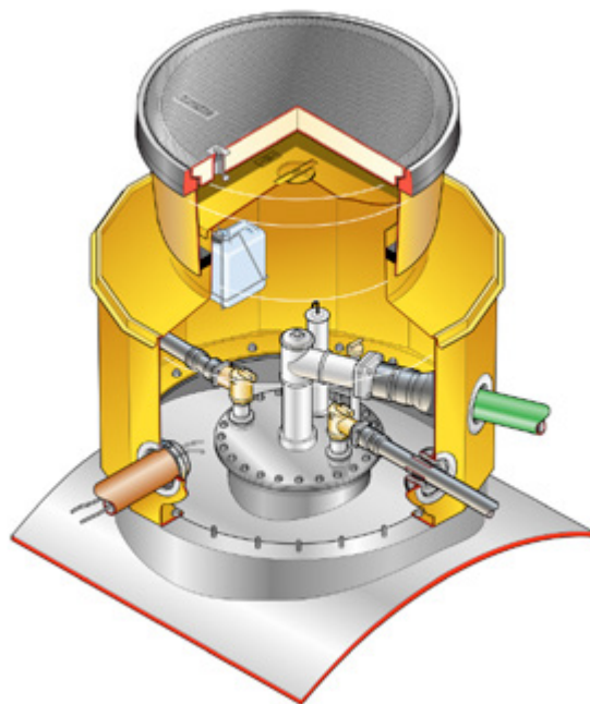
Fibrelite tank sumps are vacuum testable, ensuring liquid tightness
